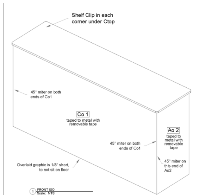
Counter Ao1, Ao2 Side Panels: 21.8125"W x 41.125"H Counter Co1 Middle Panel: 82.25"W x 41.125"H
