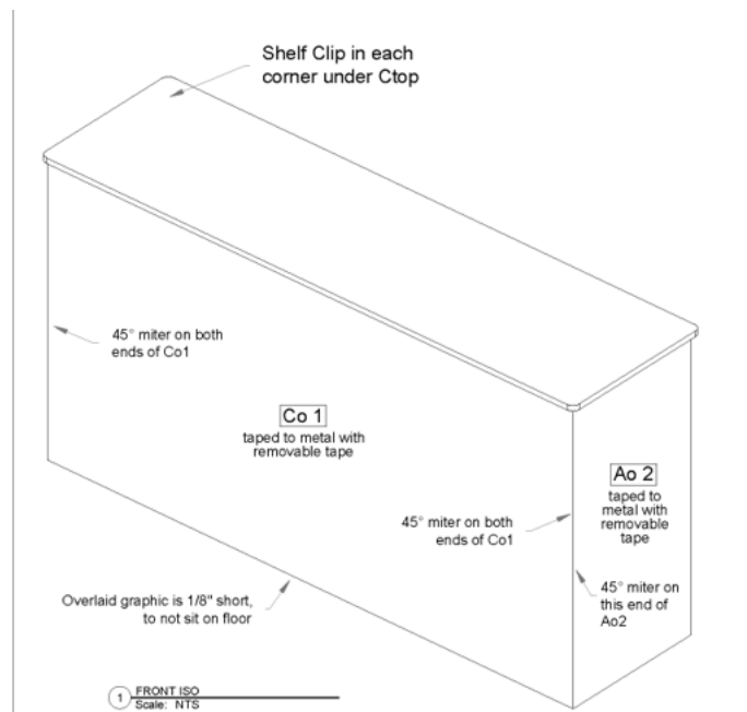
Counter Ao1, Ao2 Side Panels: 21.8125"W x 41.125"H
